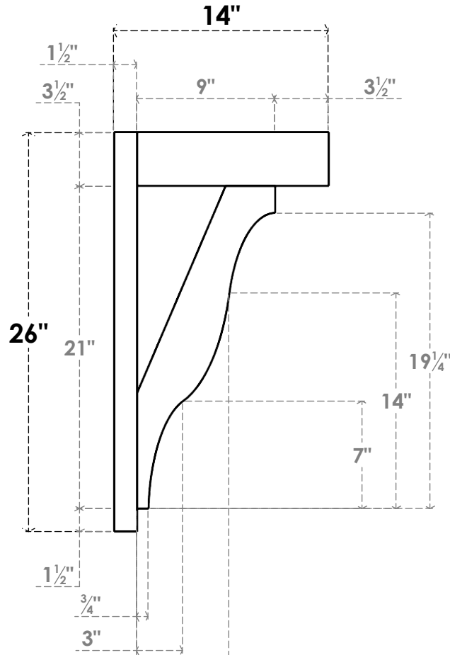
SIDE PROFILE
